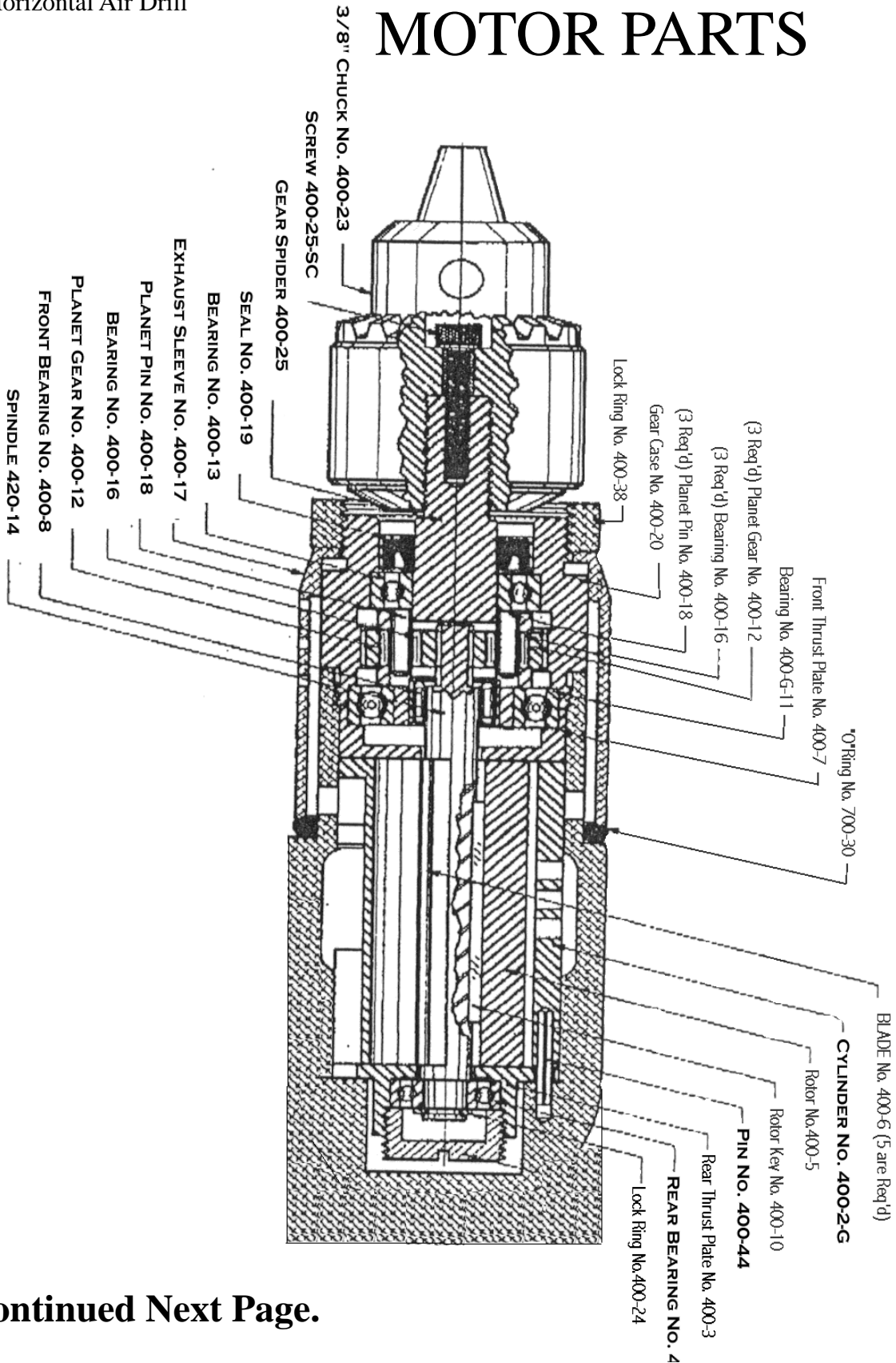
Horizontal Air Drill
